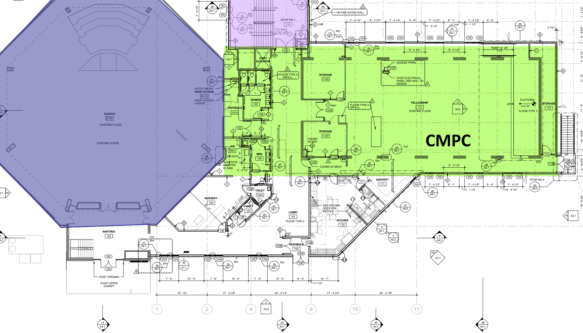
LOWER LEVEL FLOOR PLAN 1/8" = 1'-0"
